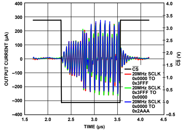
Figure 54. Digital Feedthrough
