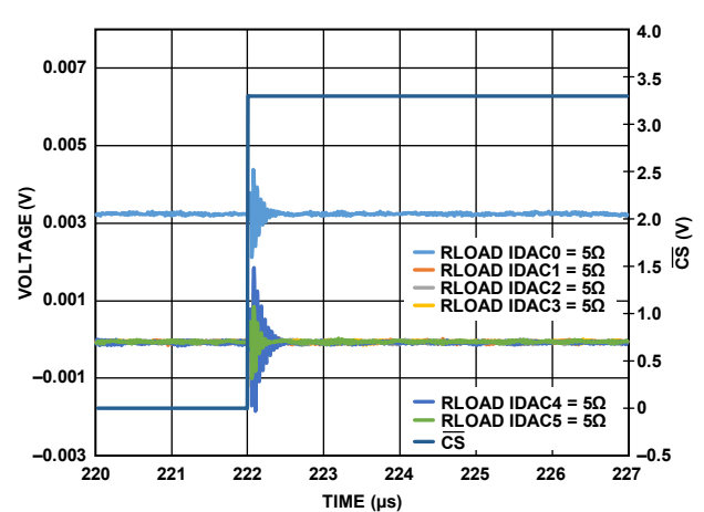
Figure 56. Analog Crosstalk
