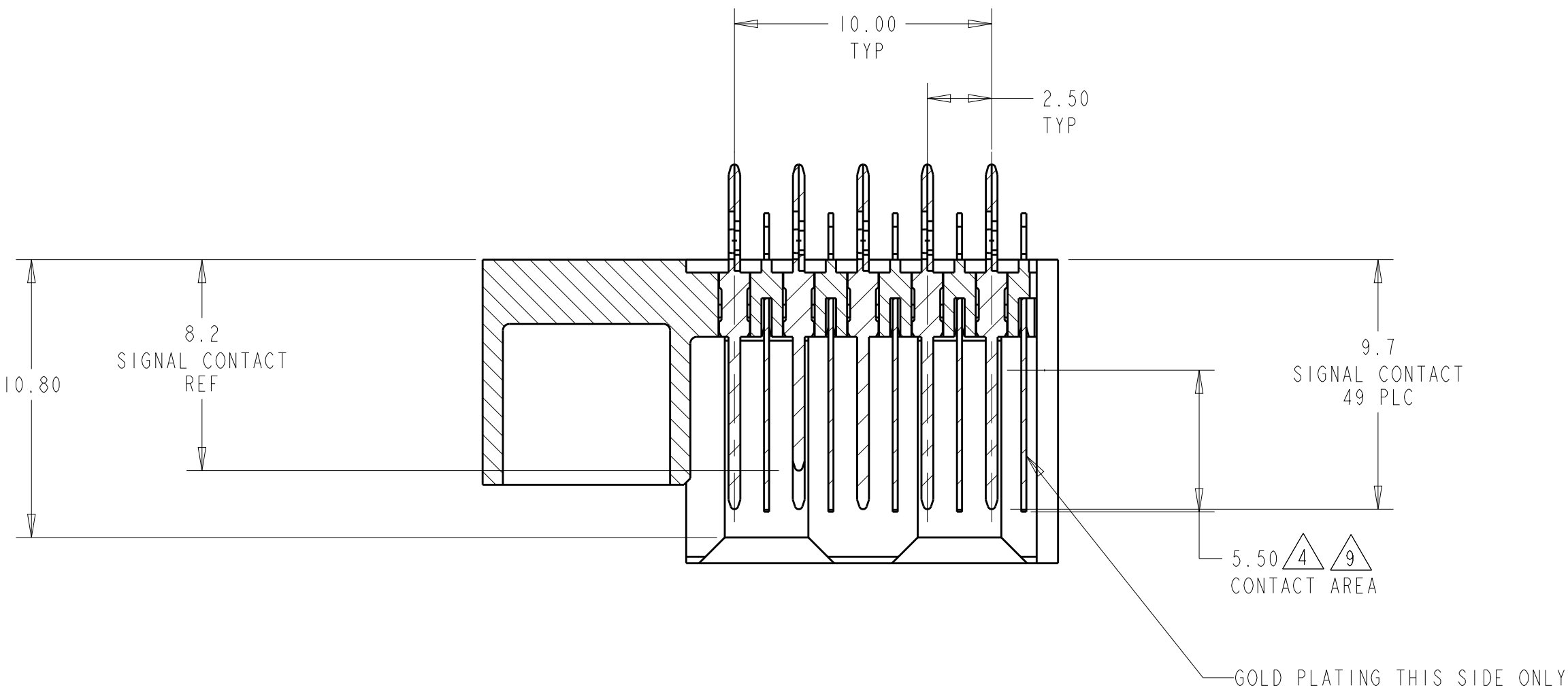
SECTION B-B
