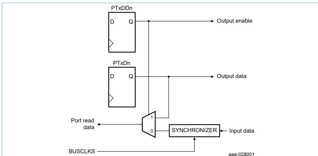
Figure 13. General purpose I/O block diagram
