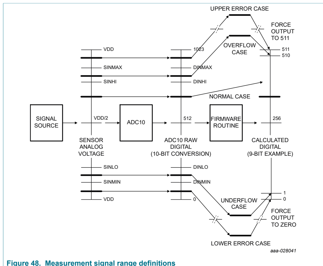
Figure 48. Measurement signal range definitions
