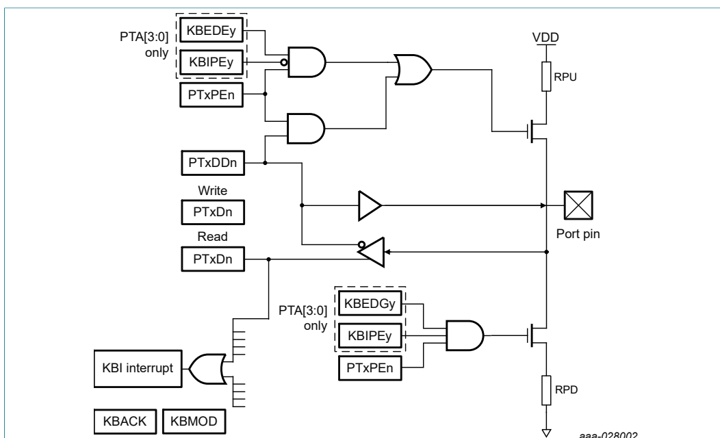
Figure 14. General purpose I/O logic
