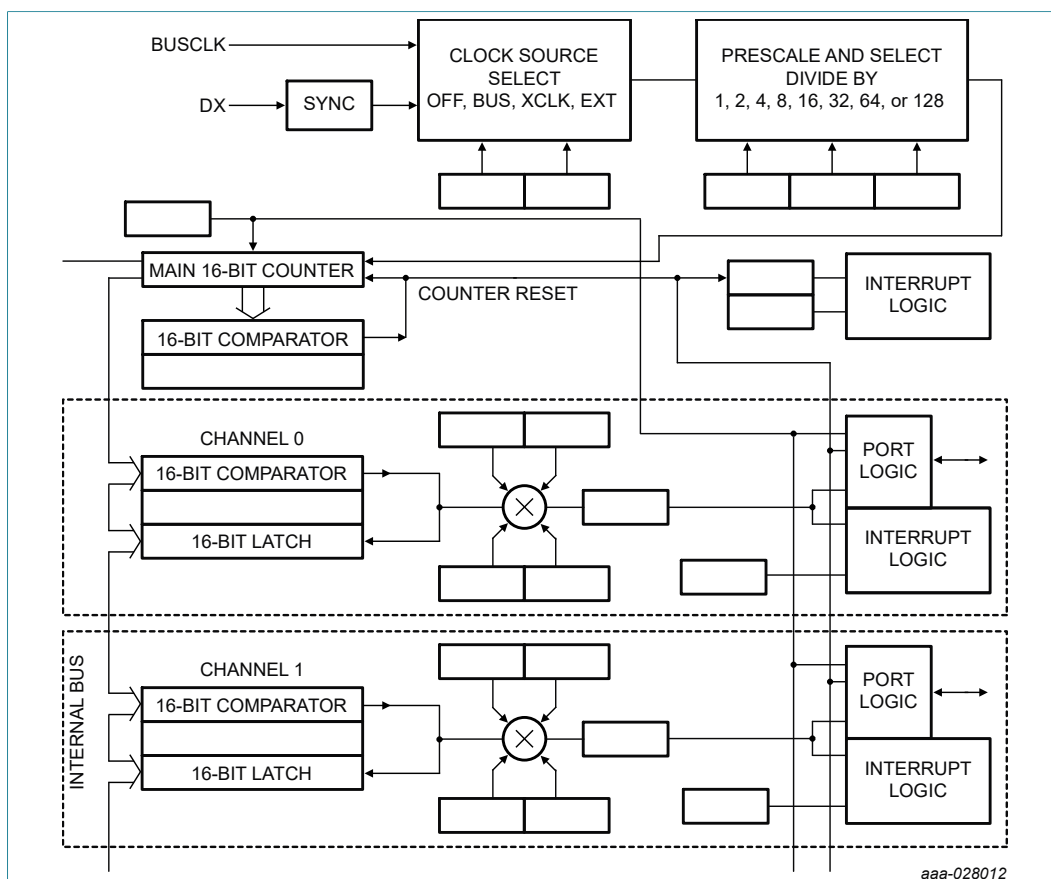
Figure 18. TPM1 block diagram
