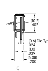
AB11 model does not have terminal 2. AB15AV-FA
