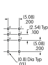
AB11 model does not have terminal 2. AB15AV-FA
