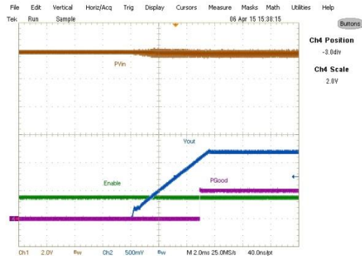
Figure 43: Operation 80, Turn ON without margining, 25A load
