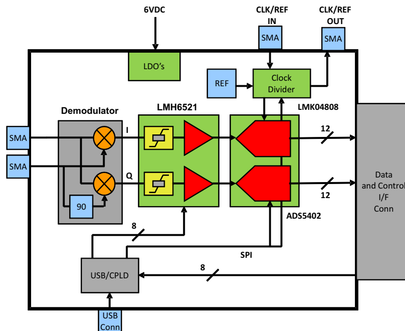
Figure 1. TSW1266EVM Block Diagram
