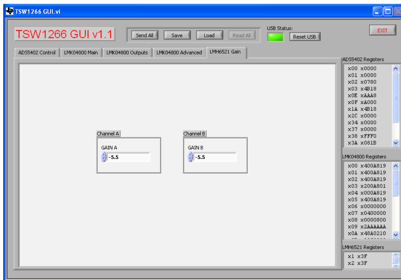
Figure 6. LMH6521 Gain Tab
