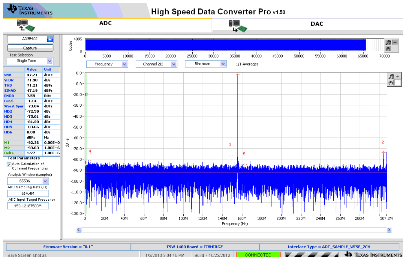
Figure 8. TSW1266 Sample Capture using the TSW1400
