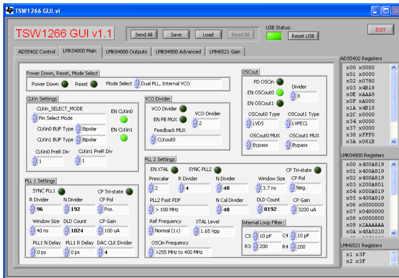
Figure 3. LMK04800 Main Tab
