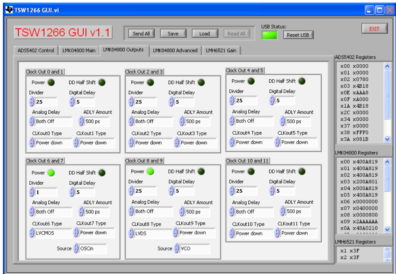
Figure 4. LMK04800 Outputs Tab
