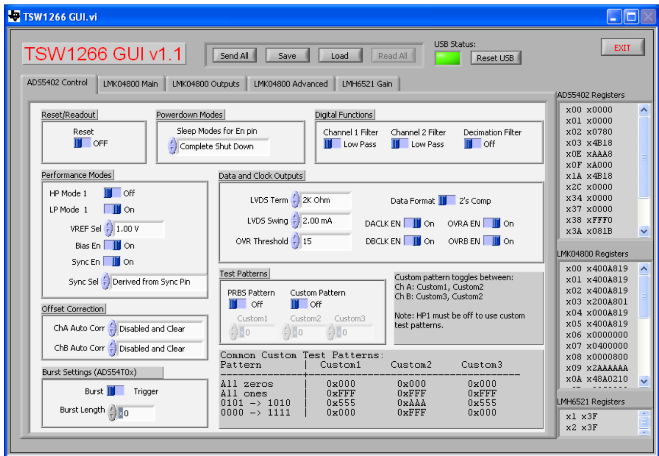
Figure 2. ADS5402 Control Tab
