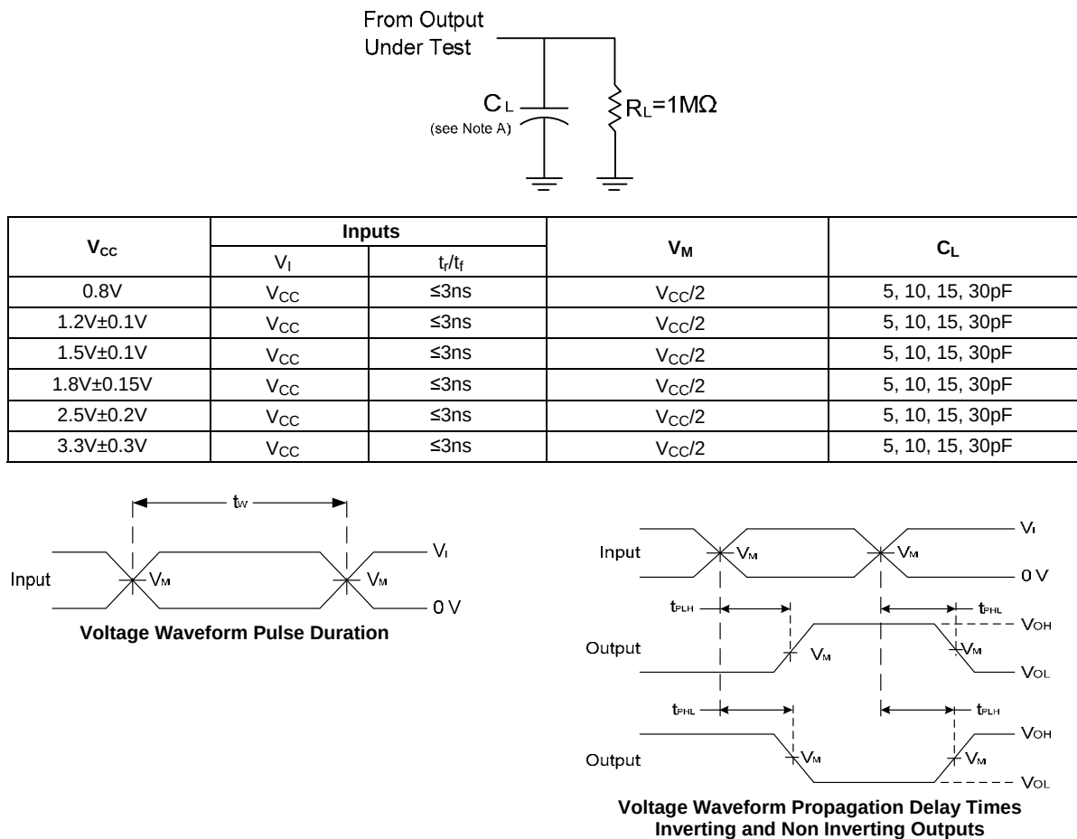
Figure 1. Load Circuit and Voltage Waveforms
