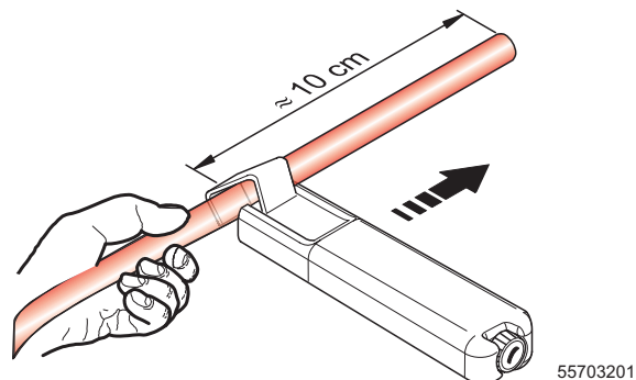
Figure 30 Stripping the outer cable sheath
