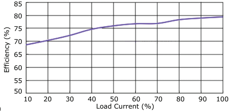
AE15-UW-S12 Efficiency Curve Efficiency vs. Load Current
