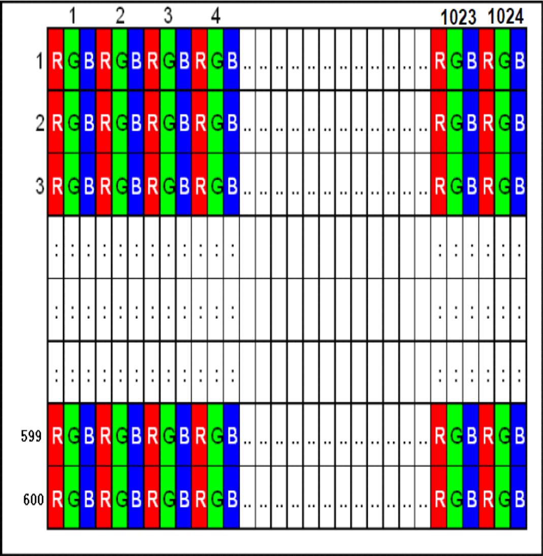
Figure 2 Pixel Format
