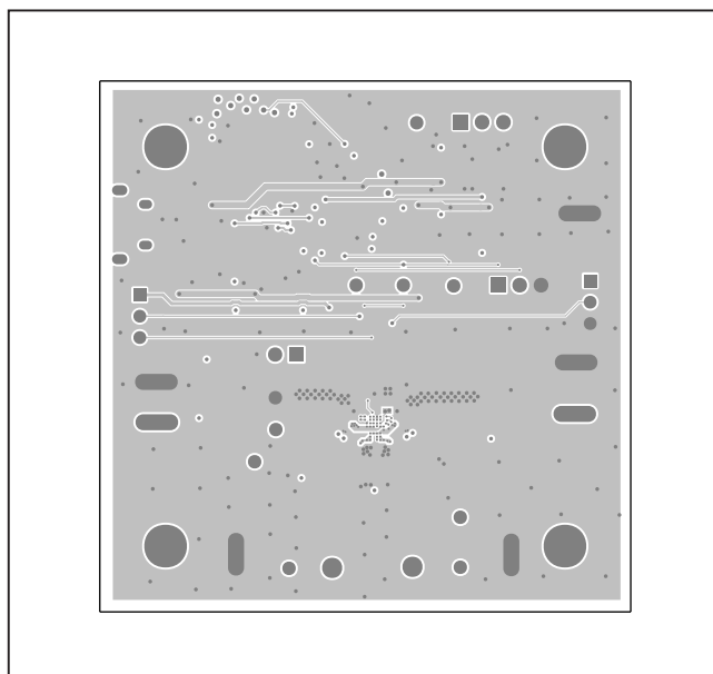
MAX77950 EV Kit PCB Layout—Internal Layer 2
