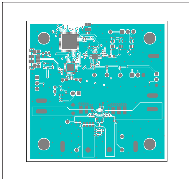
MAX77950 EV Kit PCB Layout—Top Layer
