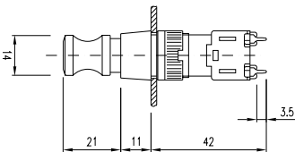
33 push-pull illuminated switch 45 mm page 607
