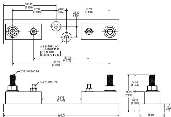
Stud-Mounted 1000 V 200 A
