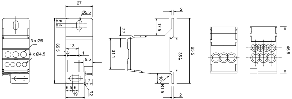
80 A GDB60801Z
