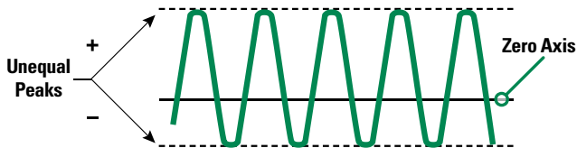
Figure 18 – Asymmetrical Current
