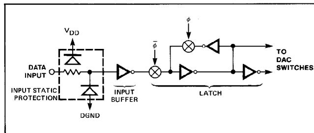
FIGURE 3: Digital Input Structure For One Bit
