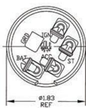
5 Screw Terminals
