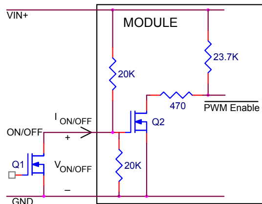
Figure 38. Circuit configuration for using positive On/Off logic.
