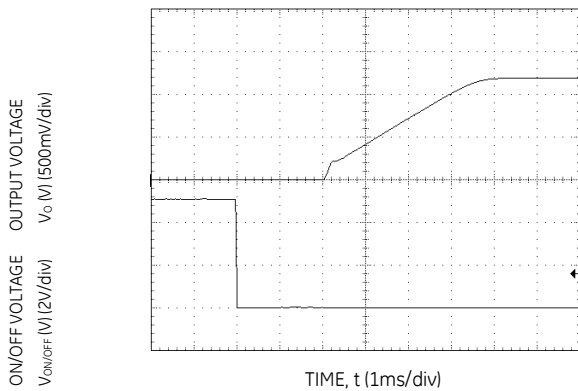
Figure 11. Typical Start-up Using On/Off Voltage (Io = Io,max).
