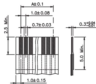
ACCOMMODATED FFC/FPC
