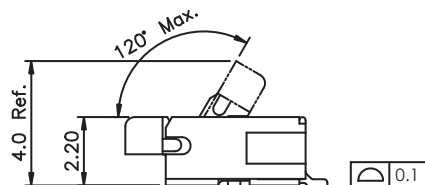
ACCOMMODATED FFC/FPC
