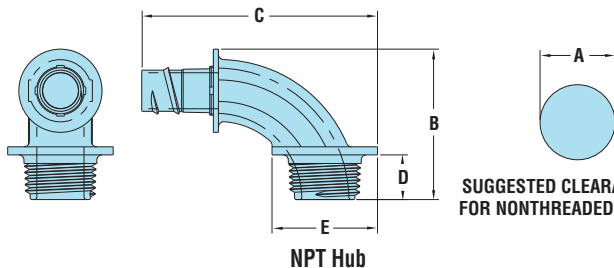
NPT Hub
