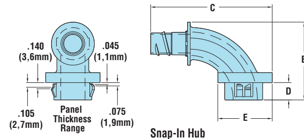
Snap-In Hub
