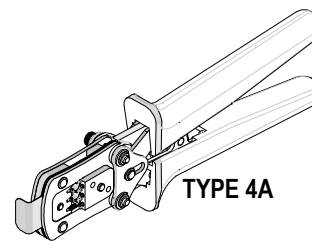
Hand Crimp Tool Order No. 63827-8900
