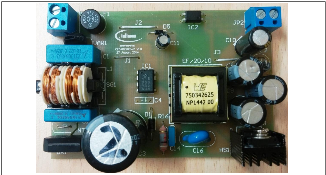
Figure 1 EVAL ICE3AR2280VJZ
