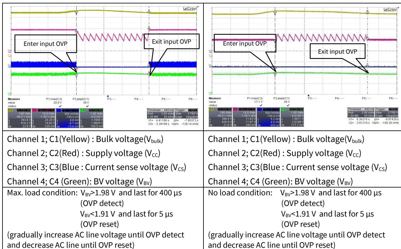
Figure 28 Input OVP
