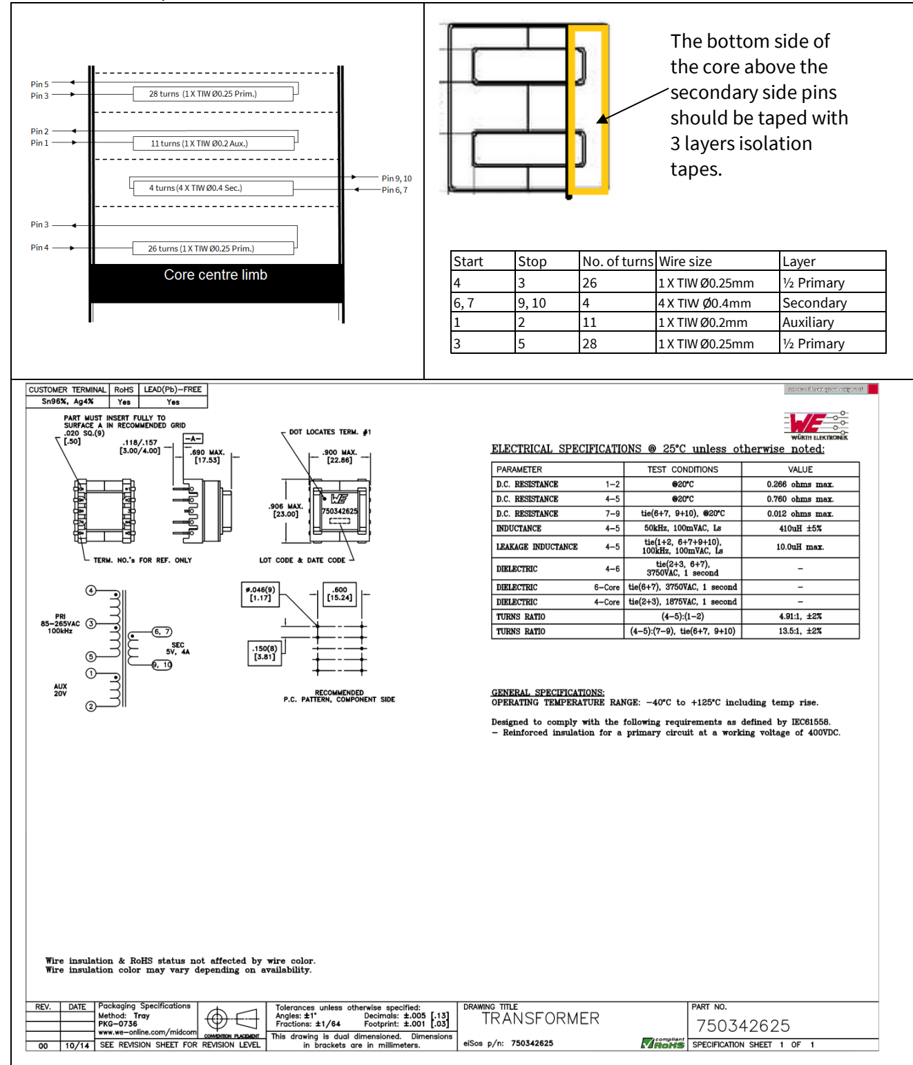
Figure 5 Transformer structure
