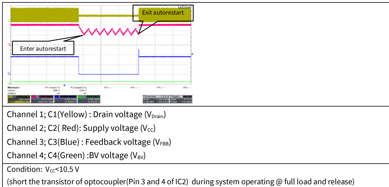
Figure 27 V_{CC} under voltage/short optocoupler protection at 85 V_{AC}
