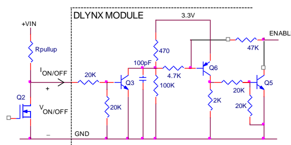
Figure 40. Circuit configuration for using negative On/Off logic.
