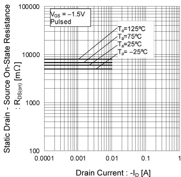
Fig.14 Static Drain - Source On - State Resistance vs. Drain Current(V)
