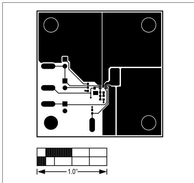
Figure 3. MAX15062C 12V EV Kit PCB Layout—Component Side
