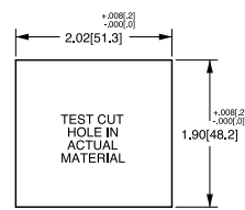
MOUNTING PANEL (2) UNITS
