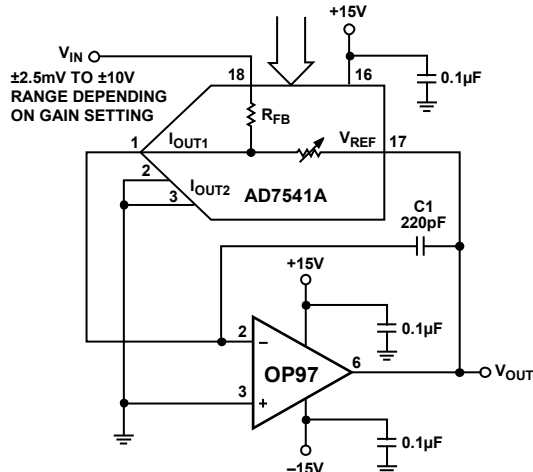
Figure 38. Precision Programmable Gain Amplifier
