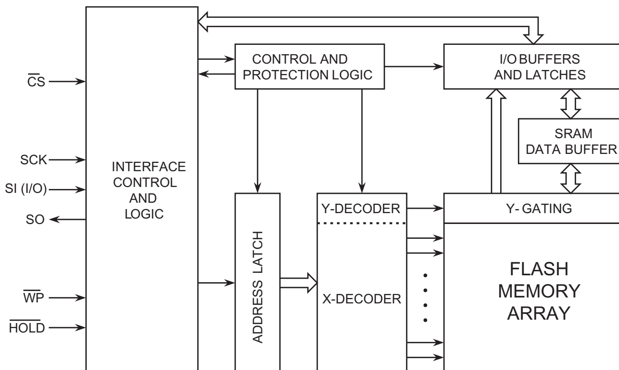
Figure 3-1. Block Diagram
