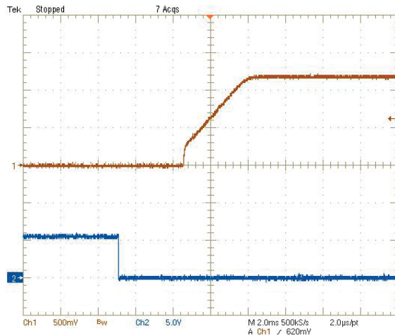
On/Off Enable Delay (Vin=12V, Vout=1.2V, Iout=20A, Cload=188μF) Trace2=Enable, 5V/div Trace1=Vout, 500mV/div
