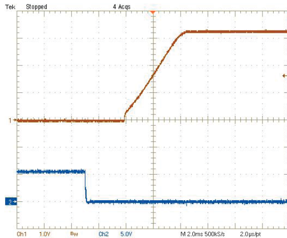
On/Off Enable Delay (Vin=12V, Vout=3.3V, Iout=20A, Cload=188μF) Trace2=Enable, 5V/div Trace1=Vout, 1V/div
