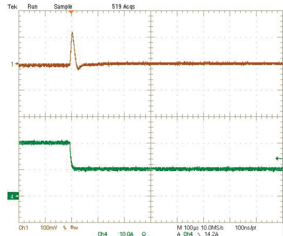
Step Load Transient Response (Vin=12V, Vout=1.2V, Cload=188μF, Iout=20A to 10A) Trace 1=Vout, 100 mV/div(AC), Trace 4=Iout, 10A/div.
