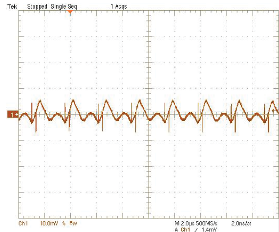
Output Ripple and Noise (Vin=12V, Vout=1.2V, Iout=20A, Cload=188μF, ScopeBW=20MHz) Trace1=Vout, 10mV/div(AC)
