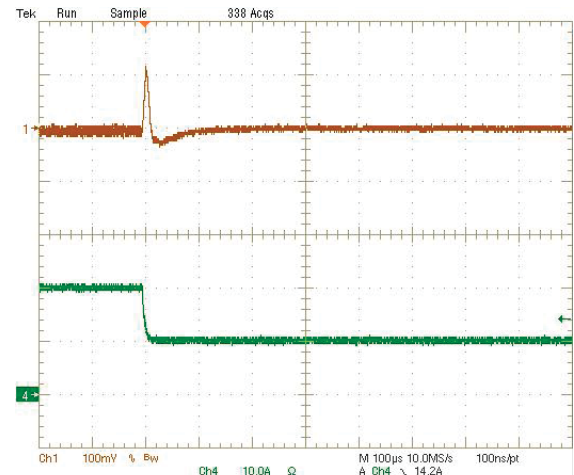
Step Load Transient Response (Vin=12V, Vout=5.0V, Cload=188μF, Iout=20A to 10A) Trace 1=Vout, 100 mV/div(AC), Trace 4=Iout, 10A/div.
