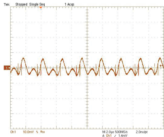
Output Ripple and Noise (Vin=12V, Vout=1.8V, Iout=20A, Cloud=188μF, ScopeBW=20MHz) Trace1=Vout, 10mV/div(AC)
