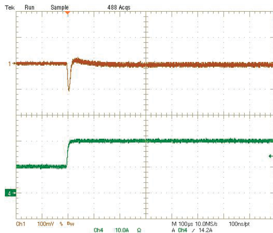
Step Load Transient Response (Vin=12V, Vout=3.3V, Cload=188μF, Iout=10A to 20A) Trace 1=Vout, 100 mV/div(AC), Trace 4=Iout, 10A/div.
