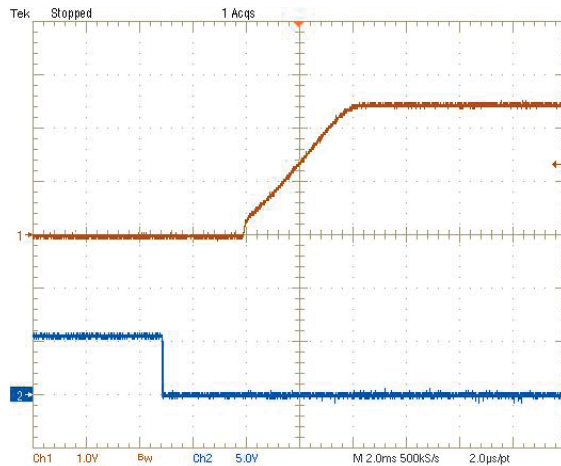
On/Off Enable Delay (Vin=12V, Vout=2.5V, Iout=20A, Cload=188μF) Trace2=Enable, 5V/div Trace1=Vout, 1V/div
