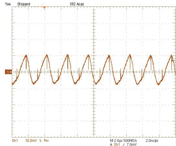
Output Ripple and Noise (Vin=12V, Vout=5.0V, Iout=20A, Cload=188μF, ScopeBW=20MHz) Trace1=Vout, 10mV/div(AC)
