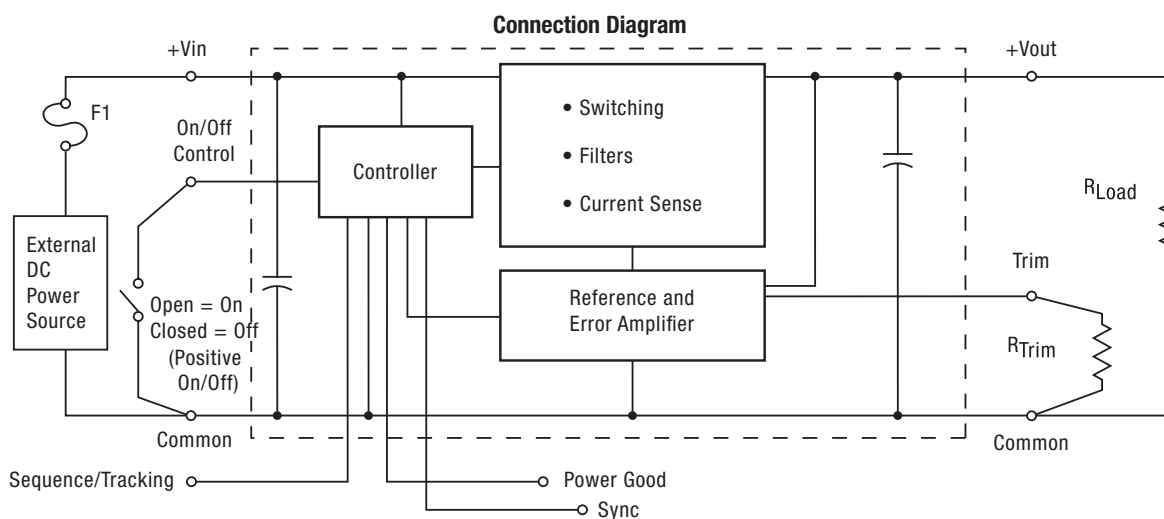
Figure 1. OKL2-T/20-W12
