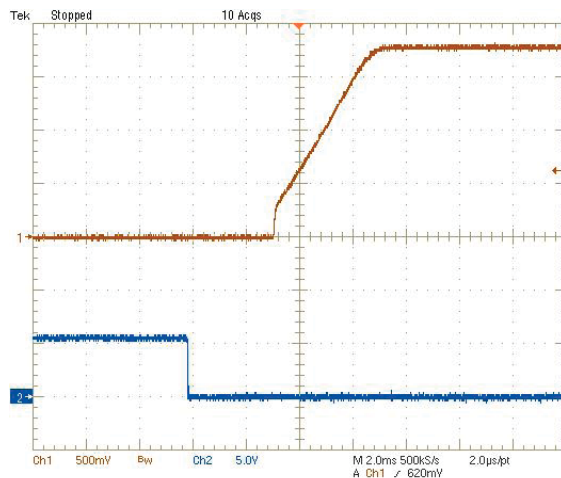
On/Off Enable Delay (Vin=12V, Vout=1.8V, Iout=20A, Cloud=188μF) Trace2=Enable, 5V/div Trace1=Vout, 500mV/div
