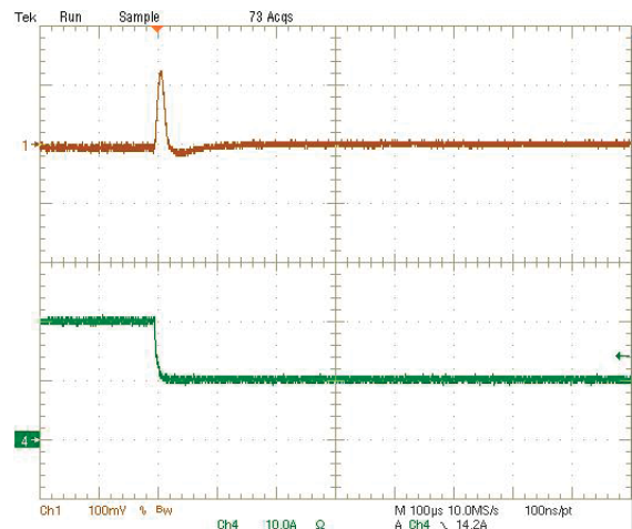
Step Load Transient Response (Vin=12V, Vout=1.8V, Cloud=188μF, Iout=20A to 10A) Trace 1=Vout, 100 mV/div(AC), Trace 4=Iout, 10A/div.
