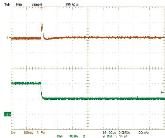
Step Load Transient Response (Vin=12V, Vout=2.5V, Cload=188μF, Iout=20A to 10A) Trace 1=Vout, 100 mV/div(AC), Trace 4=Iout, 10A/div.
