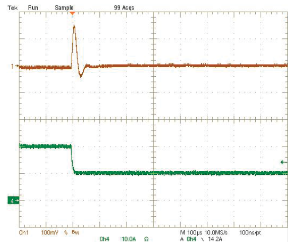
Step Load Transient Response (Vin=7V, Vout=0.69V, Load=188μF, Iout=20A to 10A) Trace 1=Vout, 100 mV/div(AC), Trace 4=Iout, 10A/div.
