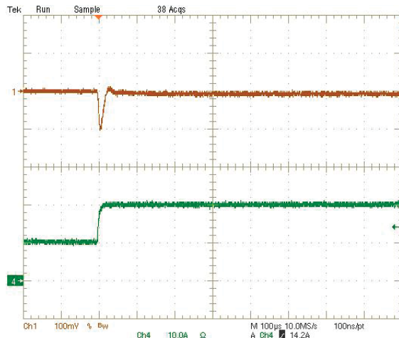
Step Load Transient Response (Vin=12V, Vout=1.2V, Cload=188μF, Iout=10A to 20A) Trace 1=Vout, 100 mV/div(AC), Trace 4=Iout, 10A/div.
