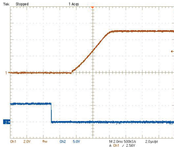
On/Off Enable Delay (Vin=12V, Vout=5.0V, Iout=20A, Cload=188μF) Trace2=Enable, 5V/div Trace1=Vout, 2V/div
