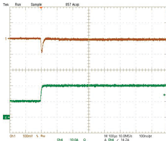
Step Load Transient Response (Vin=12V, Vout=1.8V, Cloud=188μF, Iout=10A to 20A) Trace 1=Vout, 100 mV/div(AC), Trace 4=Iout, 10A/div.
