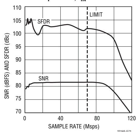
LTC2215 SNR and SFDR vs Sample Rate, f_{IN} = 5.2\text{MHz}
