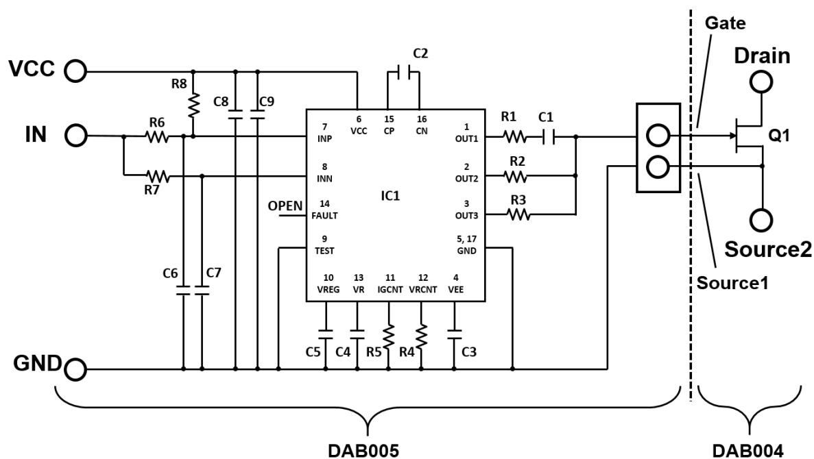
Figure 7: PGA26E19BA-DB001 schematic
