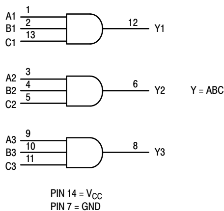
Figure 1. Logic Diagram
