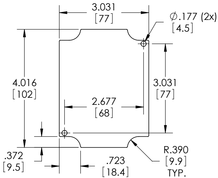
SUGGESTED PC BOARD LAYOUT
