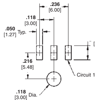
Recommended PC Board Layout * 3 Position
