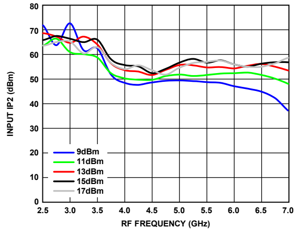
Figure 17. Input IP2 vs. RF Frequency at Various LO Powers
