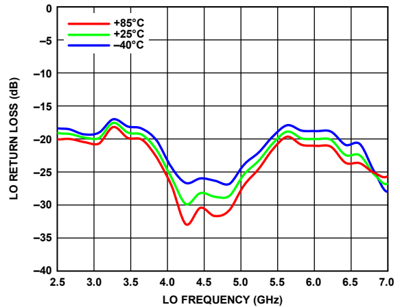
Figure 18. LO Return Loss vs. LO Frequency at Various Temperatures
