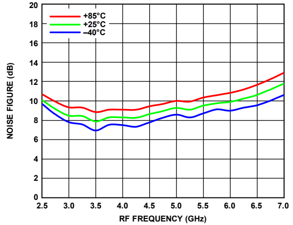
Figure 16. Noise Figure vs. RF Frequency at Various Temperatures
