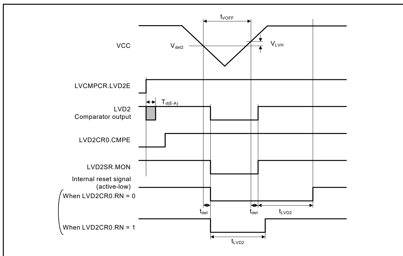
Figure 2.69 Voltage detection circuit timing ( V_{\text{det2}} )
