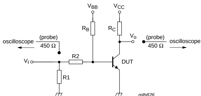
Fig 11. Test circuit for switching times
