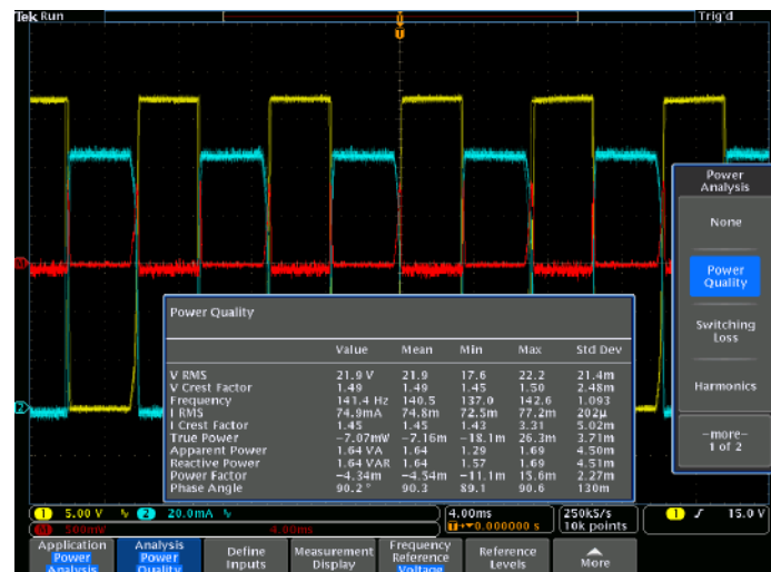
Power quality measurement. Automated power measurements enable quick and accurate analysis of common power parameters.
