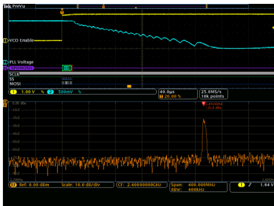
2. Spectrum Time is moved about 90 \mu s to the right. At this point, the spectrum shows that the PLL is in the process of tuning to the correct frequency (2.400 GHz). It has made it down to 2.4924 GHz.
