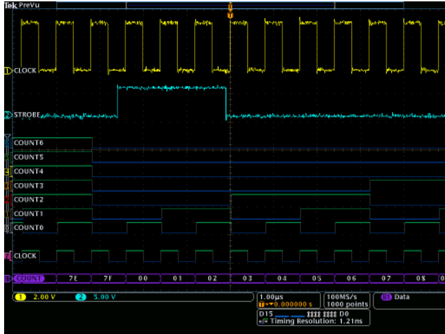
The MDO4000C Series provides 16 integrated digital channels enabling you to view and analyze time-correlated analog and digital signals.
