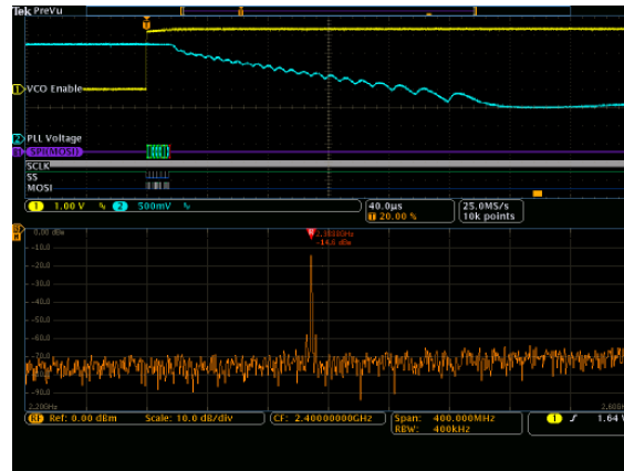
3. Spectrum Time is moved another 160 \mu s to the right. At this point the spectrum shows that the PLL has actually overshot the correct frequency and gone all the way down to 2.3888 GHz.
