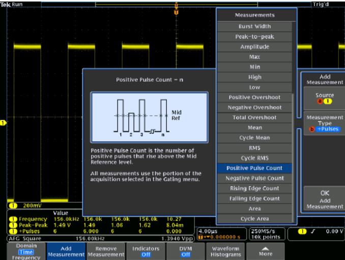
Each measurement has help text and graphics associated with it that help explain how the measurement is made.
