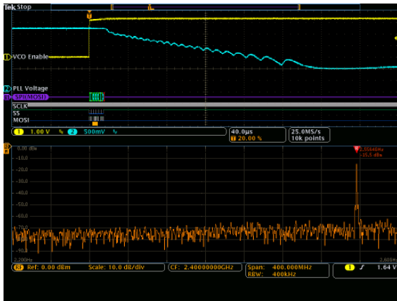
1. Time and Frequency Domain view showing the turn-on of a PLL. Channel 1 (yellow) is probing a control signal that enables the VCO. Channel 2 (cyan) is probing the VCO tune voltage. The SPI bus which is programming the PLL with the desired frequency is probed with three digital channels and automatically decoded. Notice Spectrum Time is placed after the VCO was enabled and coincident with the command on the SPI bus telling the PLL the desired frequency of 2.400 GHz. Note that the RF is at 2.5564 GHz when the circuit turns on.
