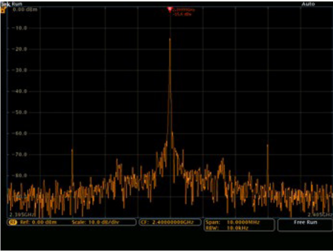
MDO4000C frequency domain display.
