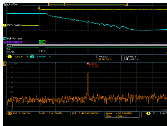
4. The PLL eventually settles on the correct 2.400 GHz frequency about 320 \mu s after the VCO was enabled.
