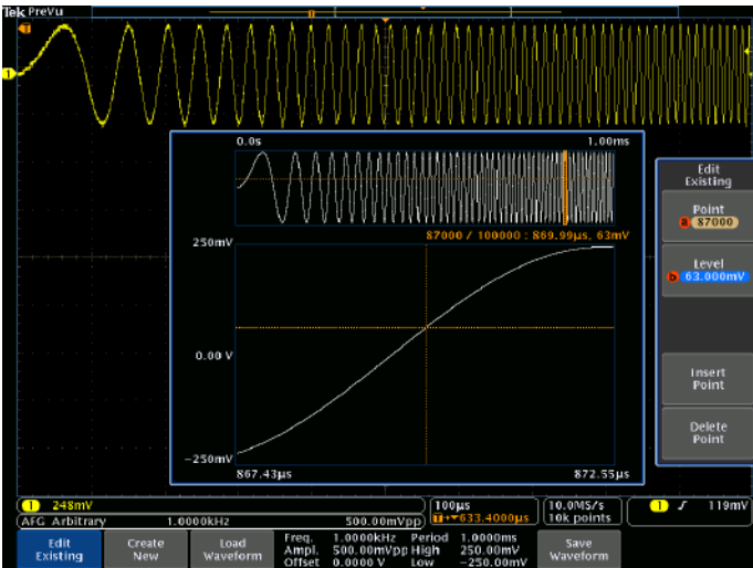
Arbitrary waveform editor showing the point-by-point editor.
