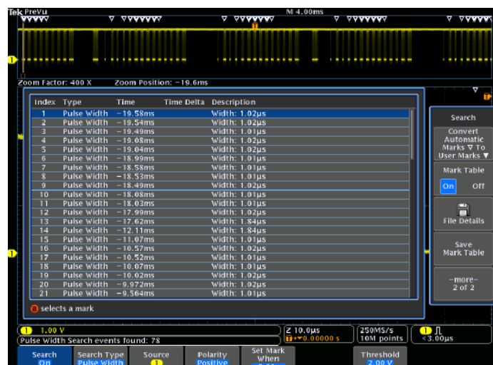
Search step 3: The Search Mark table provides a tabular view of each of the events found by the automated search. Each event is shown with a time stamp making timing measurements between events easy.
