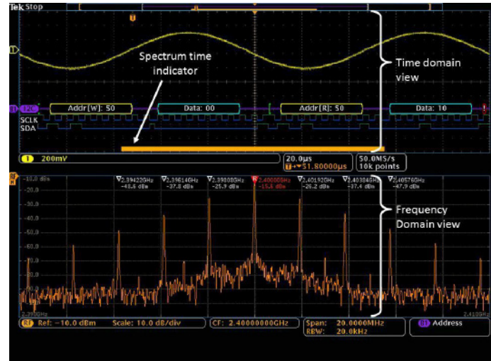
The upper half of the MDO4000C Series display shows the Time Domain view of the analog and digital channels, while the lower half shows the Frequency Domain view of the spectrum analyzer channel. The orange bar – Spectrum Time – shows the period of time used to calculate the RF spectrum.
