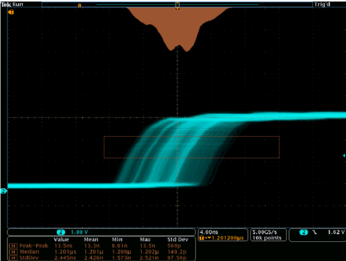
Waveform histogram of a rising edge showing the distribution of edge position (jitter) over time. Included are numeric measurements made on the waveform histogram data.
