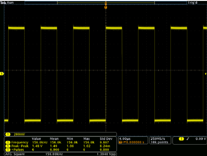
Automated measurement readouts provide repeatable, statistical views of waveform characteristics.
