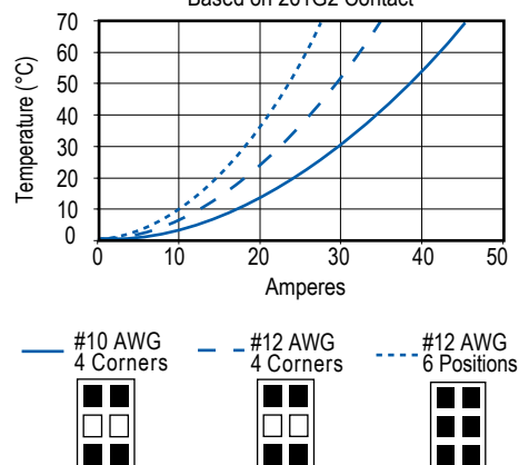
SPEC Pak® (6) Pole - Temperature Rise Based on 261G2 Contact
