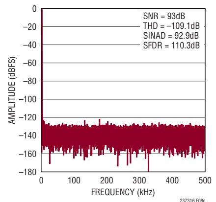
Figure 8d. 32k Point FFT f_{\text{SMP}} = 1\text{Msps} , f_{\text{IN}} = 1\text{kHz} for Circuit Shown in Figure 8a; Driven with Bipolar Inputs
