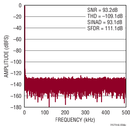
Figure 8c. 32k Point FFT f_{\text{SMP}} = 1\text{Msps} , f_{\text{IN}} = 1\text{kHz} for Circuit Shown in Figure 8a; Driven with Unipolar Inputs
