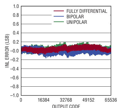
Integral Nonlinearity vs Output Code
