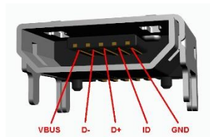
Figure 40 micro USB
