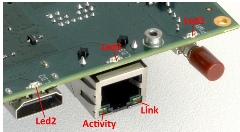
Figure 45: Carrier LEDs
