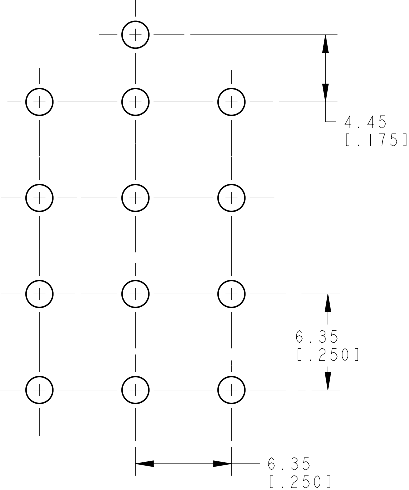
RECOMMENDED HOLE PATTERN 1.57 [0.062] THICK PC BOARD
