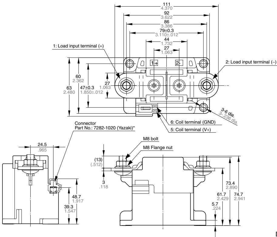
External dimensions
