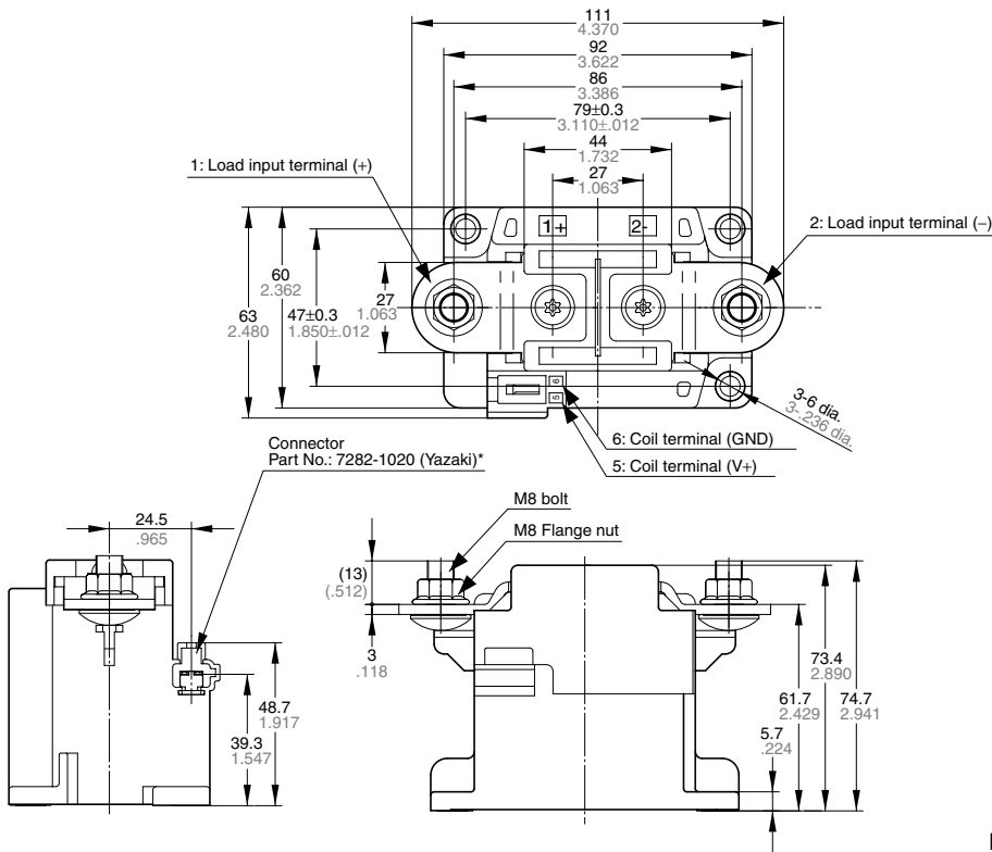
External dimensions
