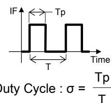
(Waveform definition)
