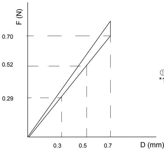
NORMAL FORCE CURVE
