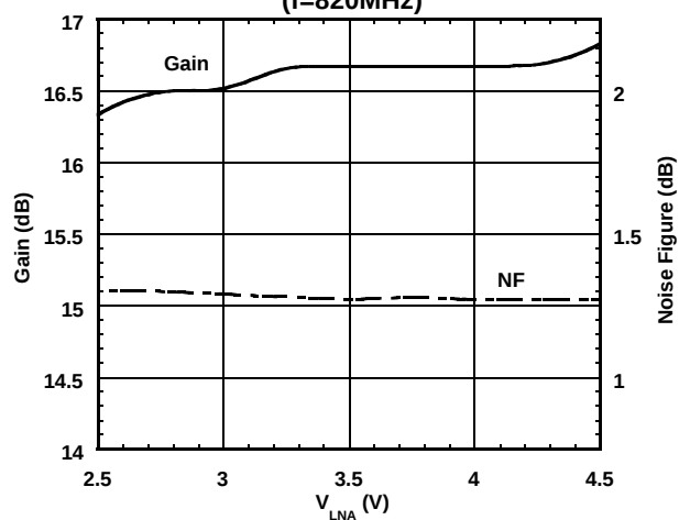
Gain, Noise Figure vs. V_{LNA}
